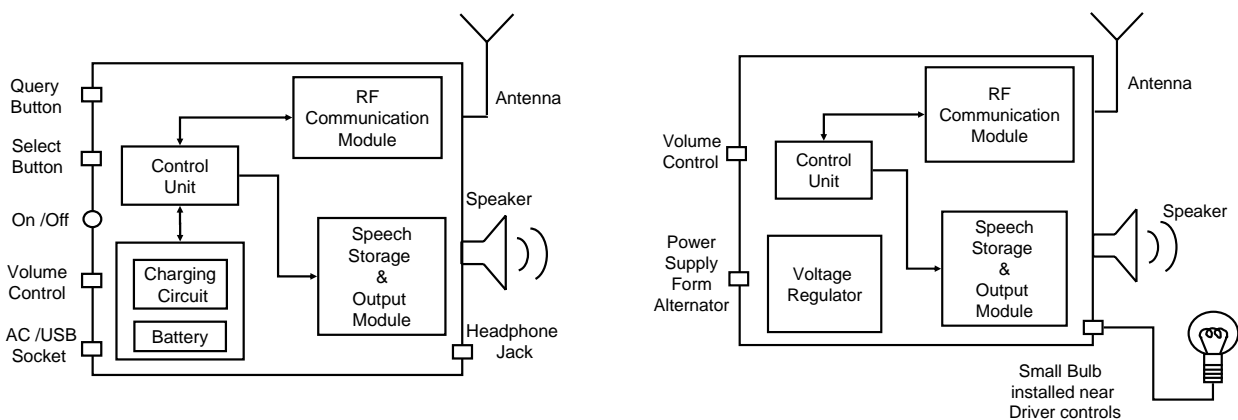
Figure 6: Top Level Block Diagram for User Module (left) and Bus Module (right)
