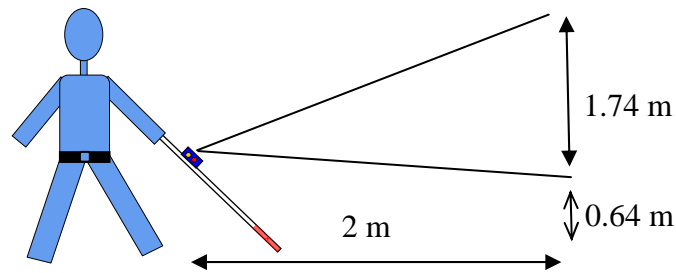
Figure 3: Side view illustrating the horizontal and vertical coverage of the detection zone at a distance of 2m from the user.
