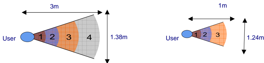
Figure 2: Top view showing the horizontal and angular coverage of the detection zone (colored) for Long Range Mode (left) and Short Range Mode (right).
